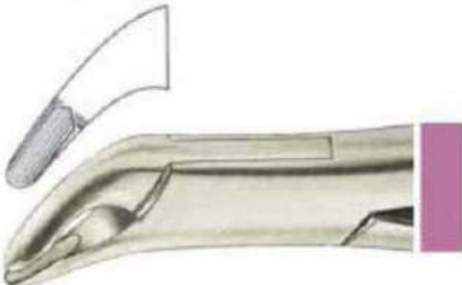
RW-092 # 151A Cryer lower incisors, premolars, roots
